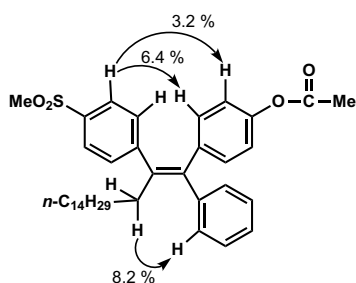
Figure 2. Some NOE determinations to determine the stereochemistry of the olefinic substituents for (Z)- 13e in \text{CDCl}_3 at 22 °C.
