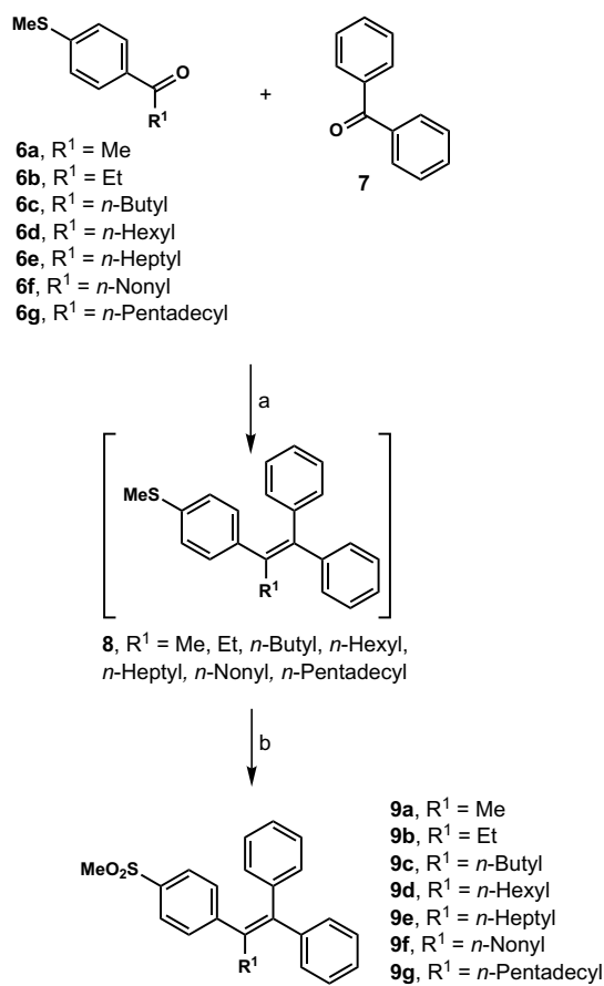
Scheme 1. Reagents and conditions: (a) Zn, TiCl 4 , THF, reflux 4.5 h; (b) Oxone ® (potassium peroxymonosulfate), MeOH, THF, H 2 O, 25°C, 15 h.
