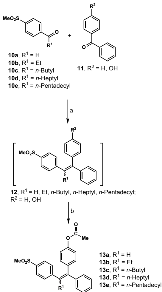
Scheme 2. Reagents and conditions: (a) Zn, \text{TiCl}_4 , THF, reflux 4.5 h; (b) AcCl, TEA, ether, 25 °C, 1.5 h.
