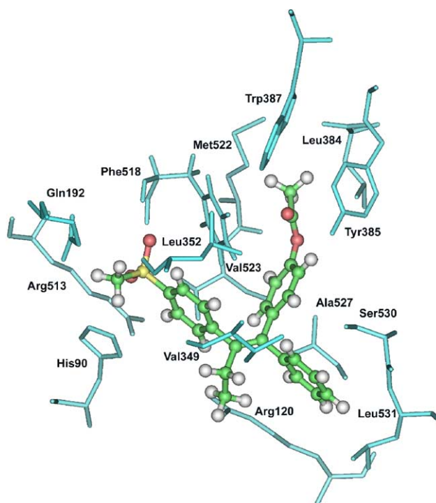
Figure 3. Docking of ( Z )- 13b in the binding site of murine COX-2. Hydrogen atoms of the amino acid residues have been removed to improve clarity.
